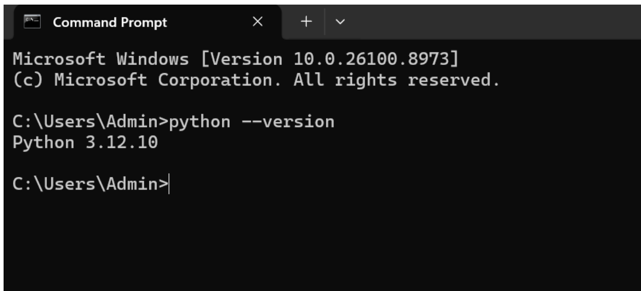
Figure.2. python version.
